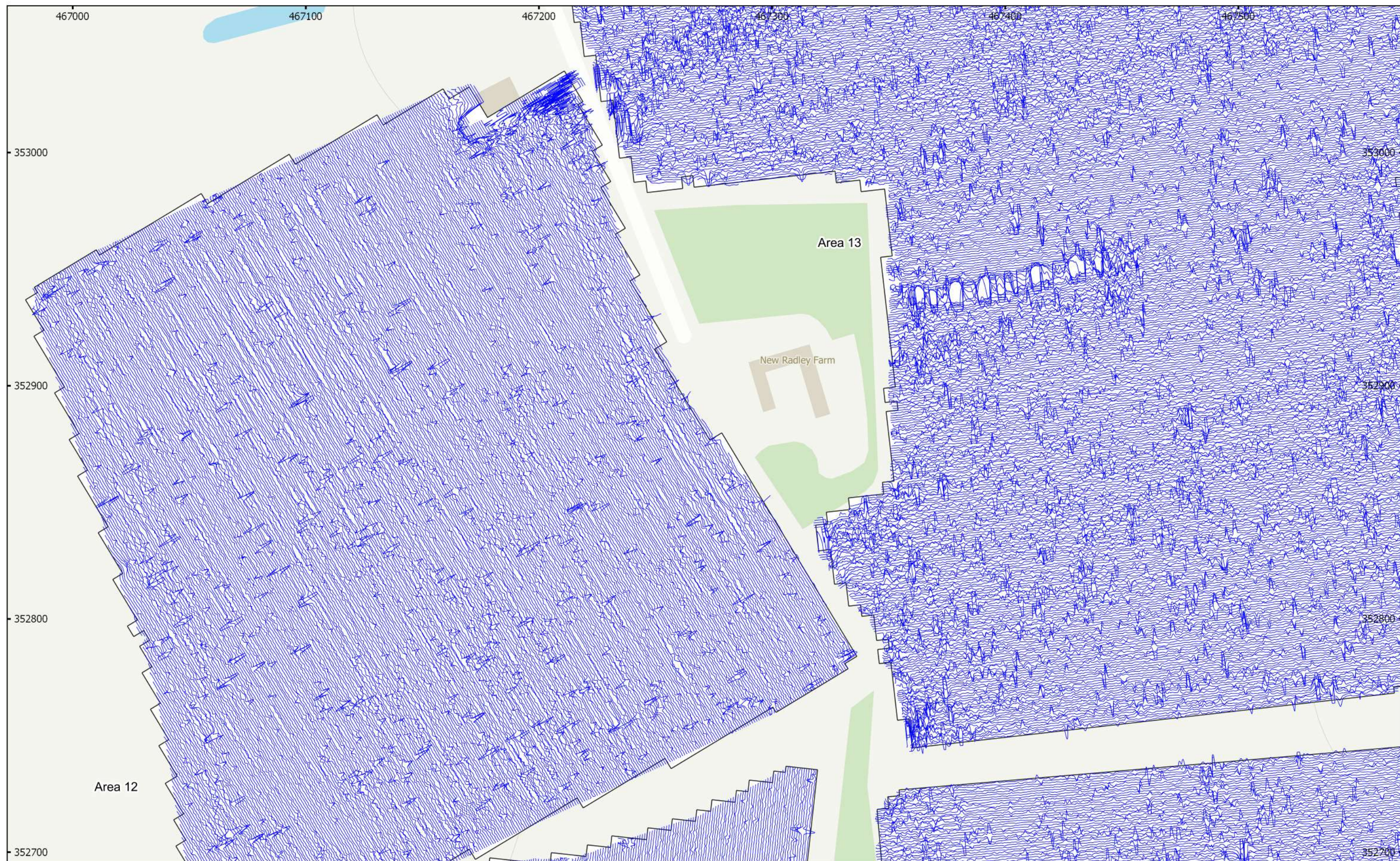
MSSK544 - Cotmoor Solar Farm Figure 32 - XY Trace Plot (Northern Area (Northwest)) 30nT/cm at 1:1,500 @ A3 Copyright Magnitude Surveys Ltd 2019 Contains Ordnance Survey data © Crown Copyright and database right 2019
