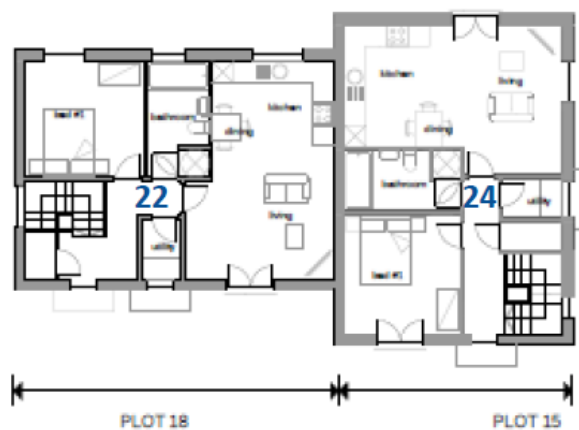
2. first floor
