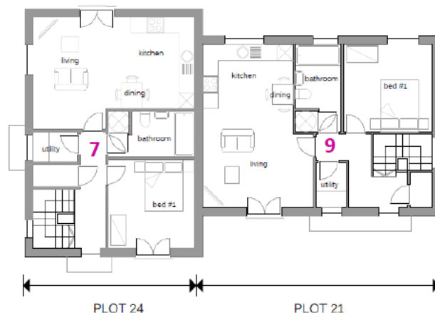
2. first floor
